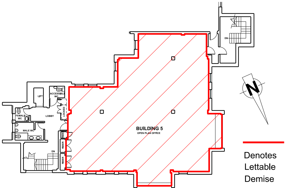
Third Floor Plan 1:200
