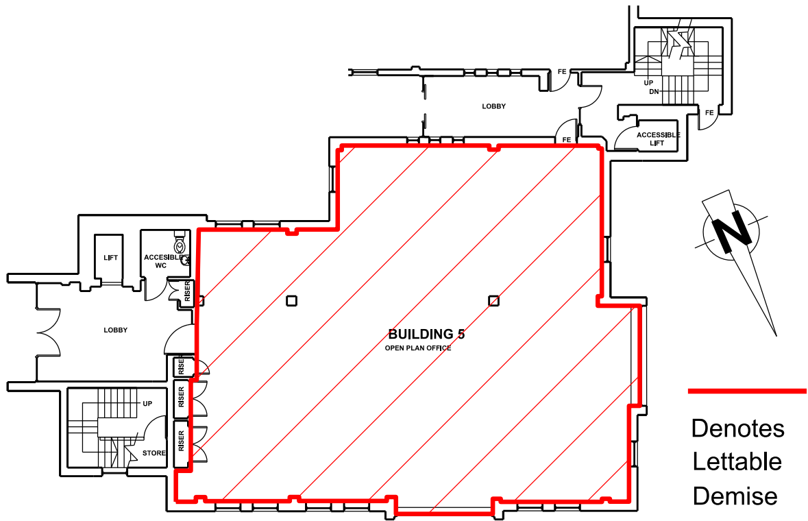
Ground Floor Plan 1:200
