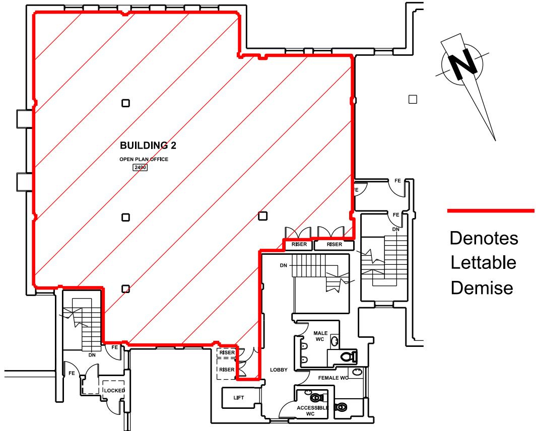
Third Floor Plan 1:200
